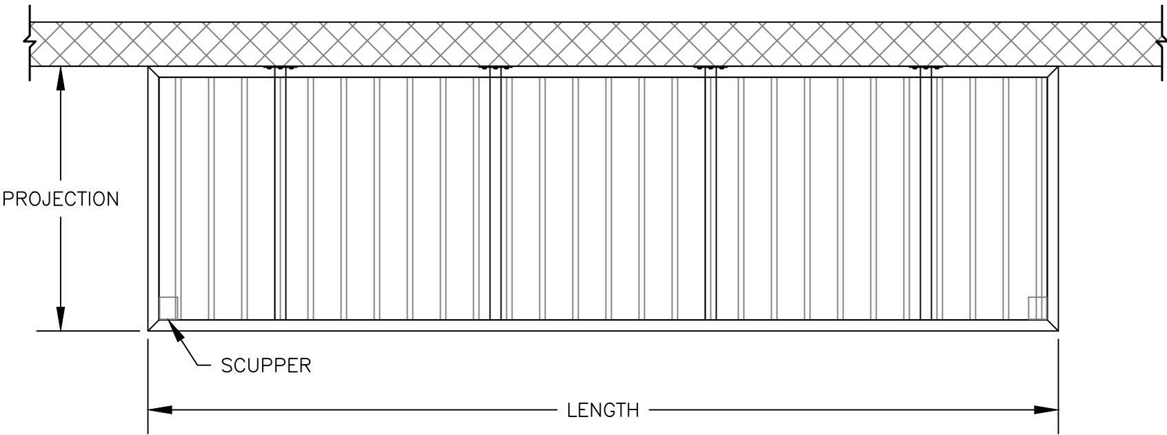
PLAN VIEW SCALE: 1/2" = 1'-0"
