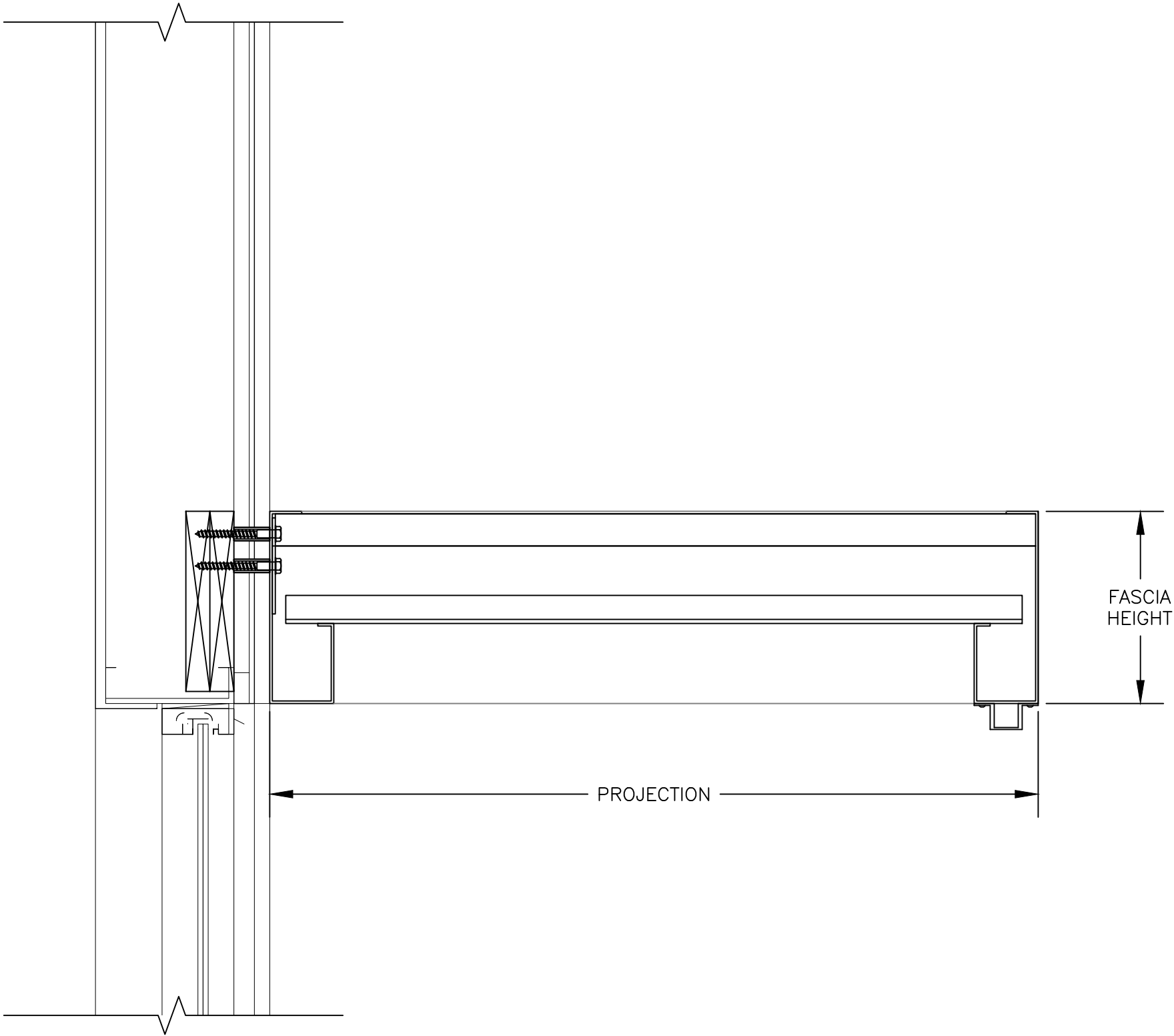
SECTION VIEW SCALE: 1 1/2" = 1'-0"
