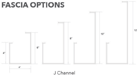
J Channel
