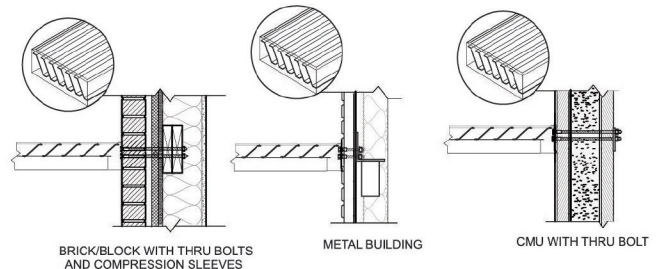
BRICK/BLOCK WITH THRU BOLTS AND COMPRESSION SLEEVES
