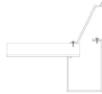
Custom Extensions for C Channel and Fascia Extensions
